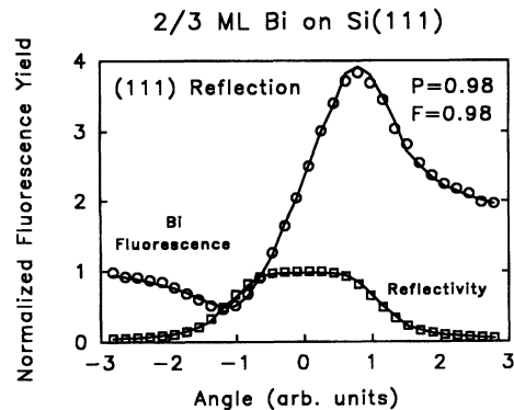
FIG. 1. The [111] reflectivity and fluorescence yield for \frac{2}{3} -ML Bi on \text{Si}(111) \sqrt{3} \times \sqrt{3} R30^\circ .
